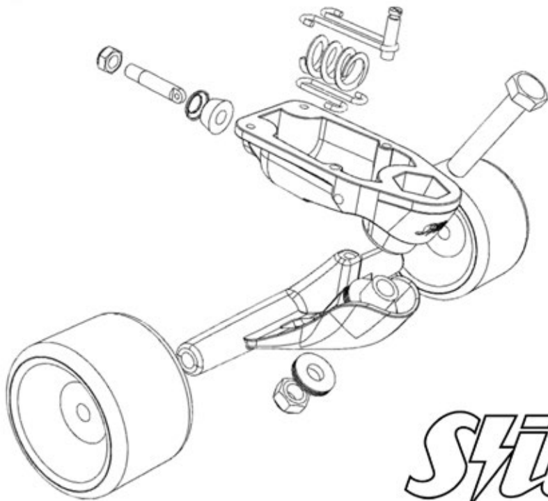
Y-ROTATION
